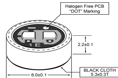
ANGLED VIEW
