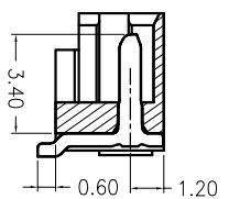
SECTION E-E
