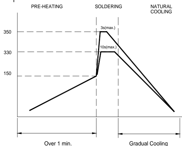
Figure 2. Hand Soldering
