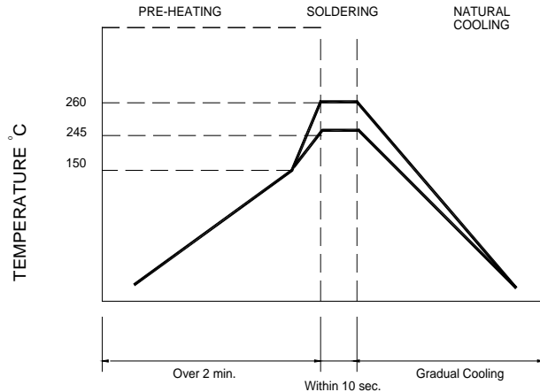
Figure 2. Wave Soldering
