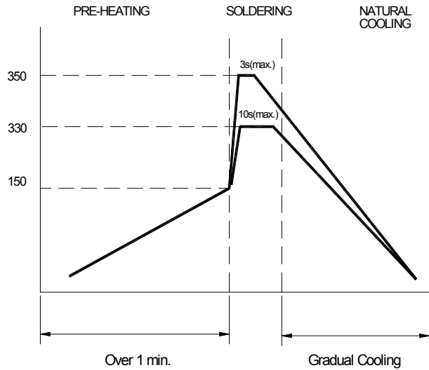
Figure 2. Hand Soldering
