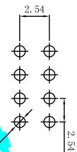
PCB Layout
