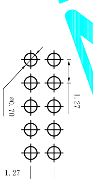
PCB Layout
