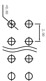
PCB Layout
