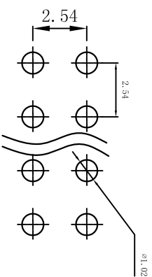
PCB Layout
