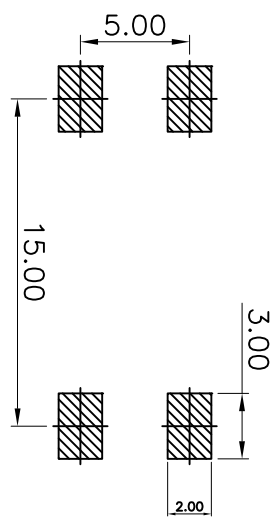
Circuit Diagram PCB Layout(Pattern side)
