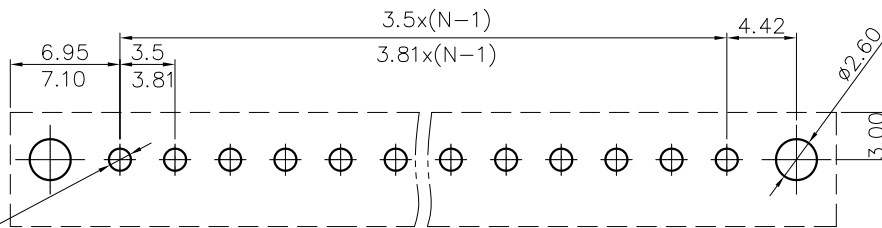
PCB LAYOUT
