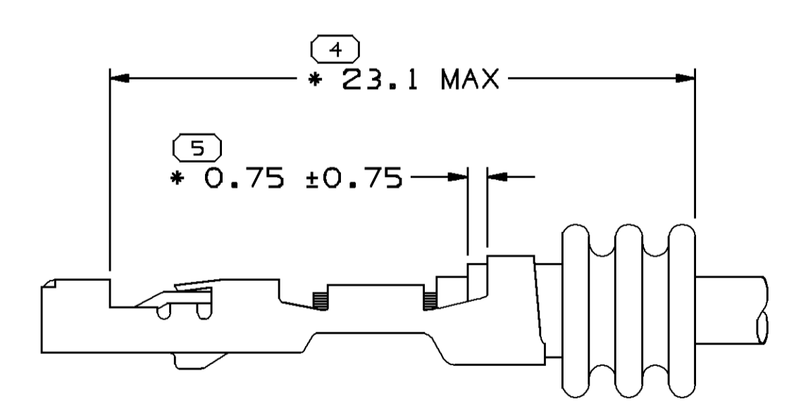
3-RIB SEAL POSITION REF SCALE 5:1
