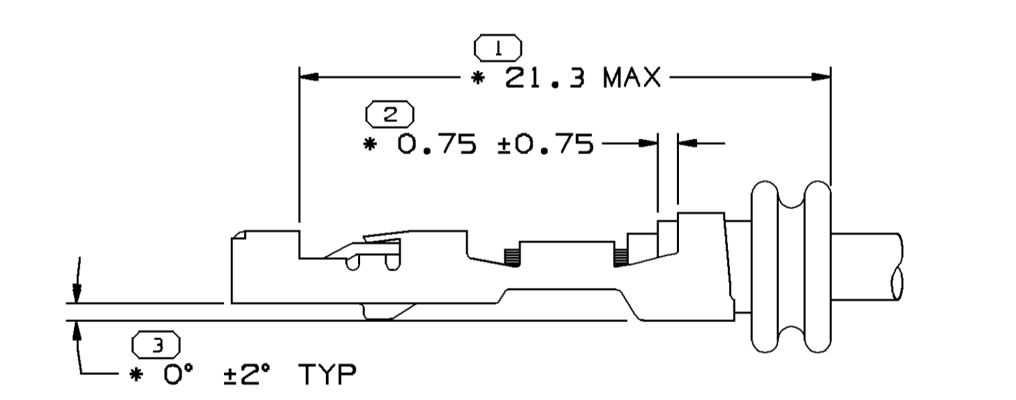
2-RIB SEAL POSITION REF AND TERMINAL/CABLE ALIGNMENT SCALE 5:1
