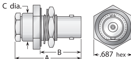
Figure 1 (Rear mount)
