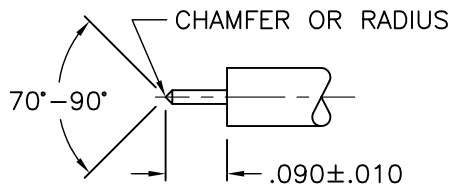
CABLE CUTTING DIMENSIONS
