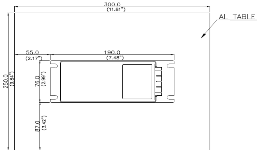
Figure 20: Thermal consideration
