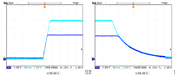
Figure 38: Sequential Start-up
