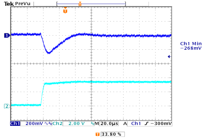
Figure 20: Typical transient response to step load change at 2.5A/µS from 50% to 100% of I_o , max at 5Vin, 3.3V out (Cout = ceramic, 10µF tantalum)
