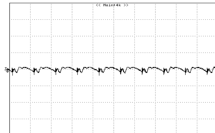
Figure 10: Output ripple & noise at 12Vin, 1.2V/5A out pk-pk: 27.08mV, rms: 5.05mV (50mV/div, 2uS/div)
