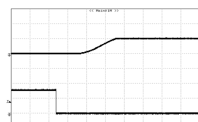
Figure 12: Turn on delay time at Remote On/Off, 5.0V/5A out (5mS/div). Top trace: Vout, 5V/div; Bottom trace: On/Off, 2V/div.
