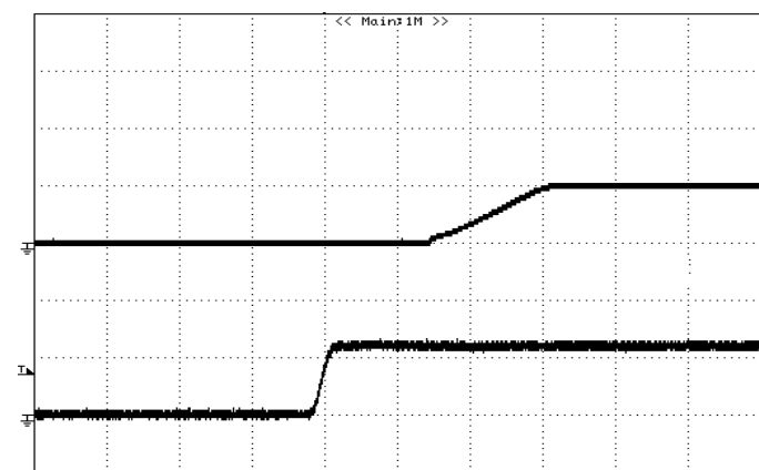
Figure 11: Turn on delay time at 12Vin, 5.0V/5A out (5mS/div), Top trace: Vout, 5V/ div; Bottom trace: Vin, 10V/div
