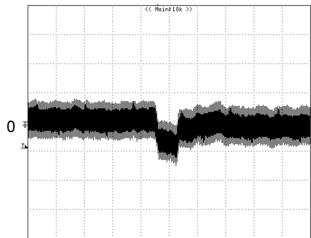
Figure 9: Output voltage response to step-change in load current (50%-75% of I_{o, \max} ; di/dt = 0.1A/\mu s ). Load cap: 10\mu F , tantalum capacitor and 1\mu F ceramic capacitor. Trace: V_{out} (20mV/div, 100us/div), Scope measurement should be made using a BNC cable (length shorter than 20 inches). Position the load between 51 mm to 76 mm (2 inches to 3 inches) from the module..
