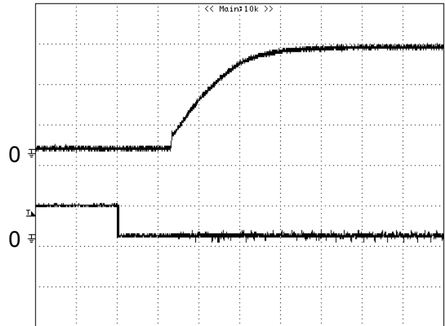
Figure 5: Turn-on transient at full rated load current (constant current load) (2 ms/div). V_{in}=48V . Top Trace: V_{out} , 1V/div; Bottom Trace: ON/OFF input, 5V/div.
