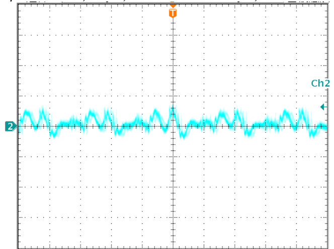
Figure 6: Output voltage ripple at Vin=72V and full load. Trace: Vout: 10mV/div, 2μs/div; Bandwidth: 20MHz.
