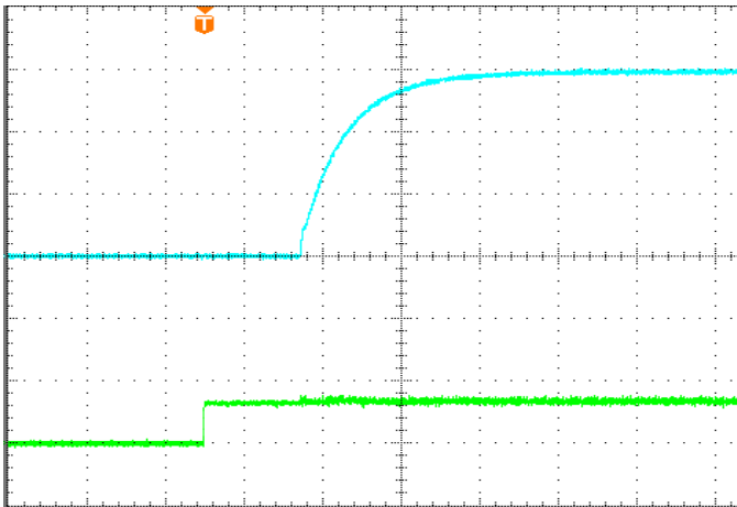
Figure 3: Turn-on transient at zero load current (20ms/div). Top Trace: Vout; 5V/div; Bottom Trace: ON/OFF input: 5V/div.
