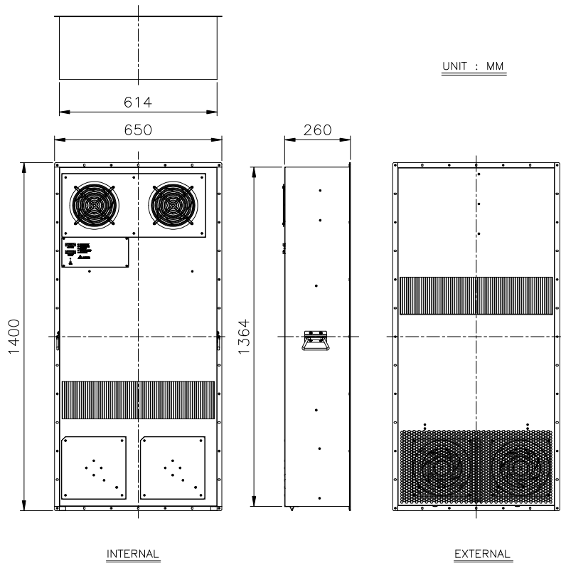
Dimension drawing
