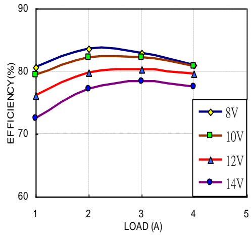
Figure 2: Converter efficiency vs. output current (1.2V output voltage)
