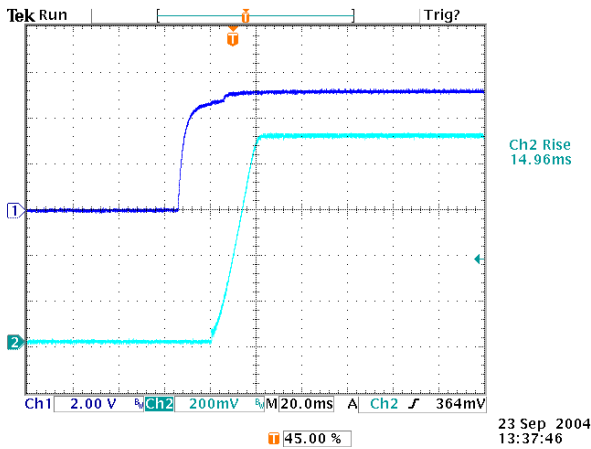
Figure 19: Remote turn on delay time at 12vin, 0.9V/4A out
