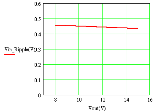
Figure 18: Input ripple voltage for various output models, I_o = 3A ( C_{in} = 2 \times 100\mu F electrolytic capacitors 1x3.3µF ceramic capacitors at the input)
