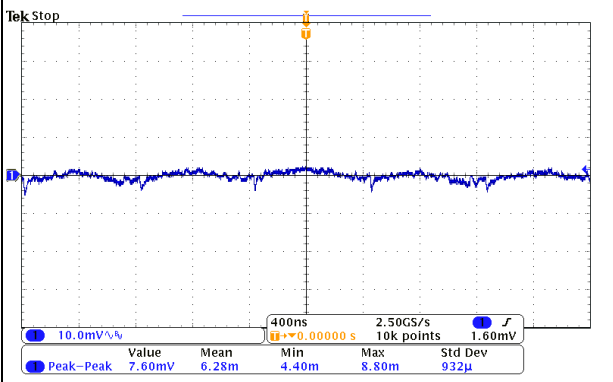
FIG.6 OUTPUT RIPPLE (12V VIN, IOU=1 A)
