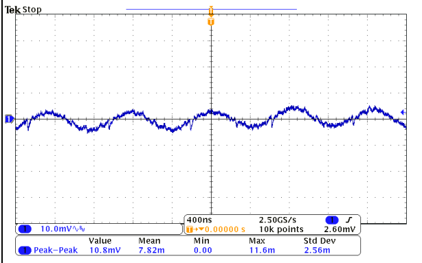
FIG.24 OUTPUT RIPPLE (12V VIN, IOUT=1 A)
