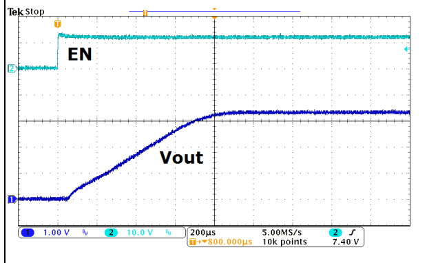
FIG.20 TURN-ON (12V VIN, IOU=1 A)
