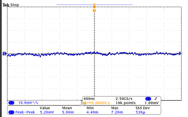
FIG.5 OUTPUT RIPPLE (12V VIN, IOU=0 A)
