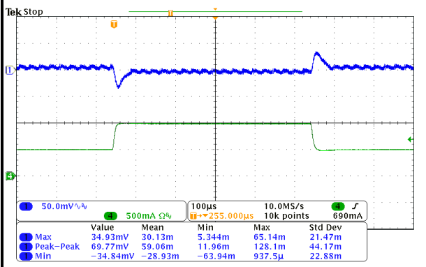
FIG.19 TRANSIENT RESPONSE (12V VIN, 0% to 100% LOAD STEP)
