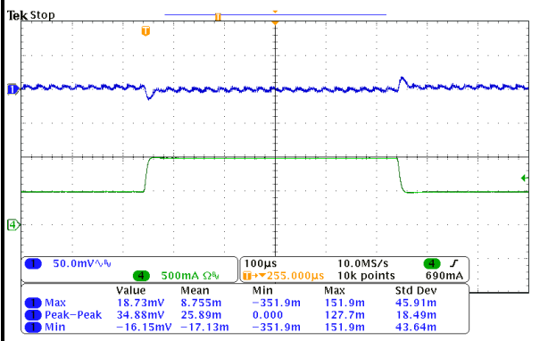
FIG.7 TRANSIENT RESPONSE (12V VIN, 50% to 100% LOAD STEP)
