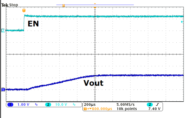
FIG.8 TURN-ON (12V VIN, IOU=1 A)
