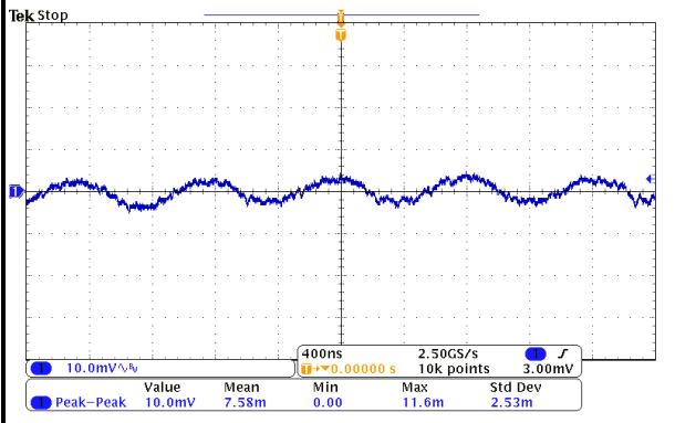
FIG.23 OUTPUT RIPPLE (12V VIN, IOUT=0 A)
