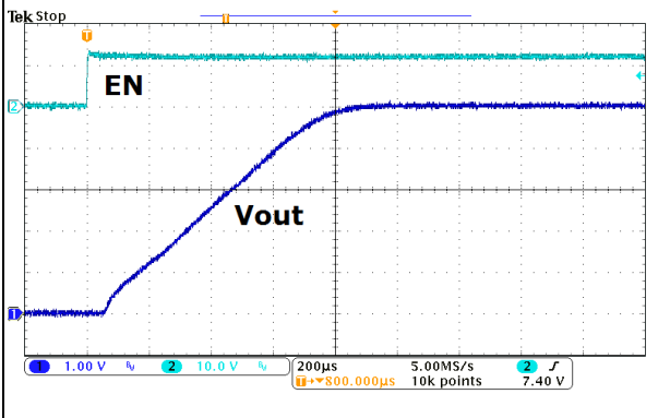
FIG.26 TURN-ON (12V VIN, IOUT=1 A)
