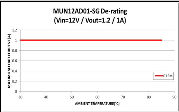
FIG.4 DE-RATING CURVE AT 12V VIN
