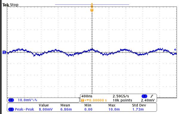
FIG.17 OUTPUT RIPPLE (12V VIN, IOU=0 A)
