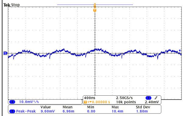
FIG.18 OUTPUT RIPPLE (12V VIN, IOU=1 A)
