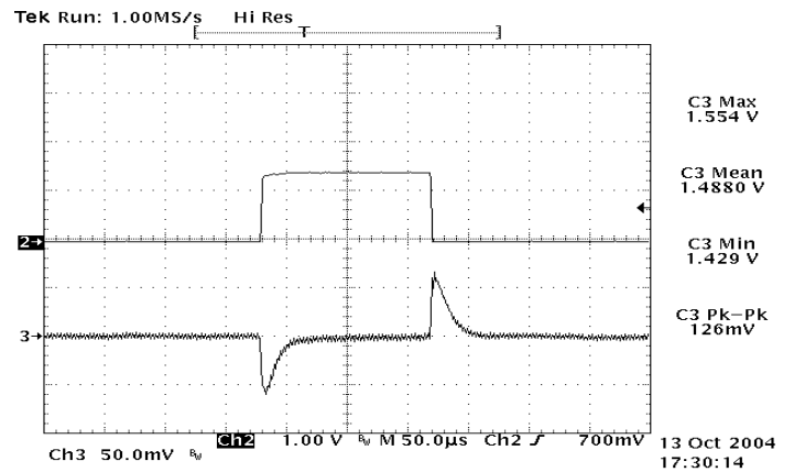
Figure 20: Typical transient response to step load change at 10A/μs from 75% to 50% of I_o , max at 12Vin, 1.5V out (Cout = 1uF ceramic, 10μF tantalum)
