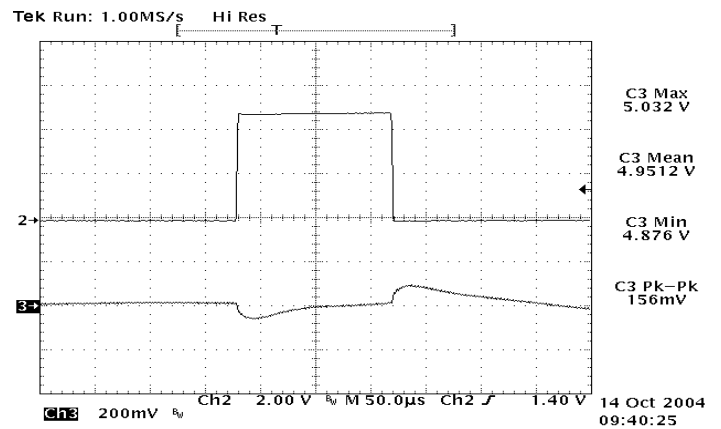
Figure 24: Typical transient response to step load change at 10A/μs from 75% to 50% of I_o , max at 12Vin, 5.0V out (Cout = 1uF ceramic, 10μF tantalum)
