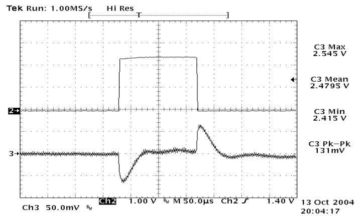
Figure 22: Typical transient response to step load change at 10A/μs from 75% to 50% of I_o , max at 12Vin, 2.5V out (Cout = 1uF ceramic, 10μF tantalum)
