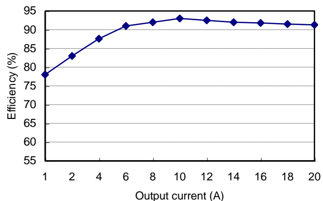
Figure 4: Converter efficiency vs. output current (2.5V output voltage, 12V input)
