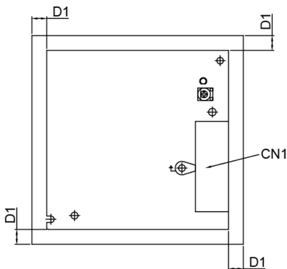
Fig. 3 Assembly Reference
