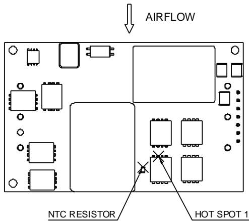
Figure 22: * Hot spot 1 & NTC resistor temperature measured points. The allowed maximum hot spot 1 temperature is defined at 118 °C
