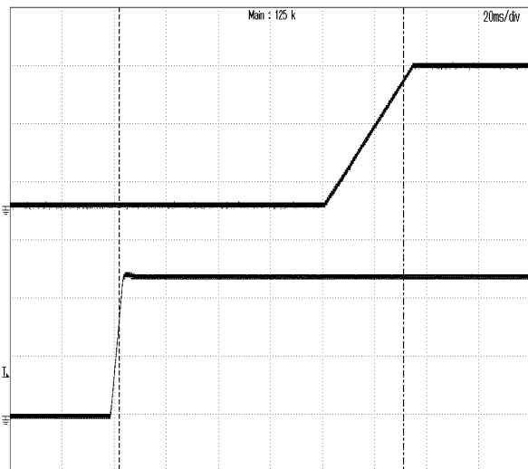
Figure 7: Turn-on transient at zero load current (20 ms/div). V_{in}=48V . Top Trace: V_{out} , 5V/div, Bottom Trace: input voltage, 20V/div
