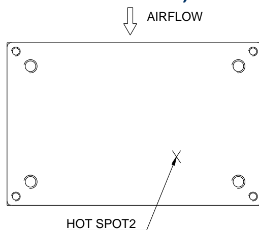
Figure 23: * Hot spot2 temperature measured point. The allowed maximum hot spot2 temperature is defined at 108°C.
