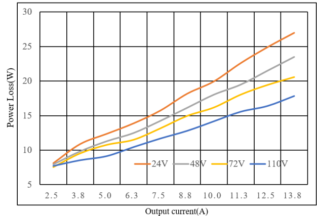
Figure 8: Power loss vs. load current at 25°C.
