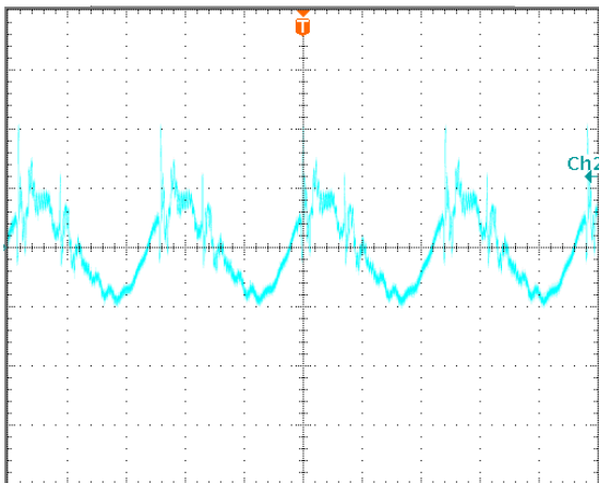
Output voltage ripple at nominal input voltage and max load current (20 mV/div, 2μs/div) Load cap: 10μF, tantalum capacitor and 1μF ceramic capacitor. Bandwidth: 20 MHz.
