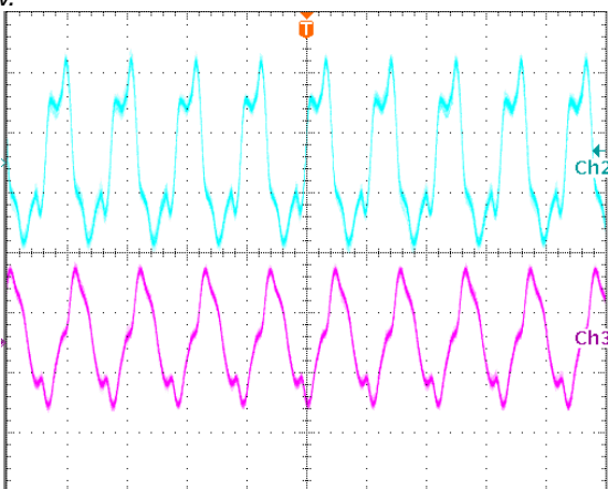
Output voltage ripple at nominal input voltage and max load current Top trace +15V, 10 mV/div, Bottom trace -15V, 20mV/div, 2us/div. Load cap: 10μF, tantalum capacitor and 1μF ceramic capacitor. Bandwidth: 20 MHz.
