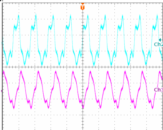
Output voltage ripple at nominal input voltage and max load current Top trace +15V, 10 mV/div, Bottom trace -15V, 20mV/div, 2us/div. Load cap: 10μF, tantalum capacitor and 1μF ceramic capacitor. Bandwidth: 20 MHz.
