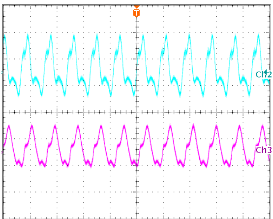
Output voltage ripple at nominal input voltage and max load current Top trace +12V, 10mV/div, Bottom trace -12V, 20mV/div, 2μs/div.
