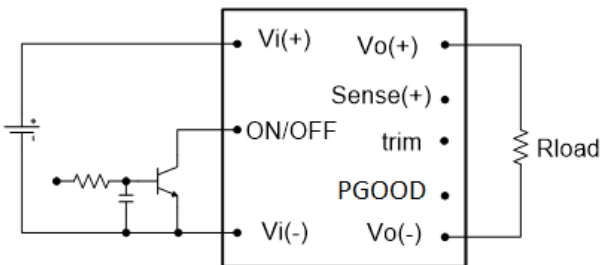
Figure 25: Remote On/Off Implementation
