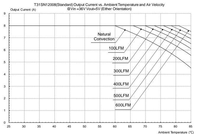
Figure 30: Output current vs. ambient temperature and air velocity @ V_{in}=36V , V_{out}=5V (Either Orientation, Open Frame)
