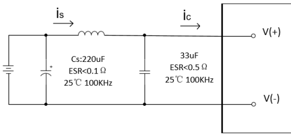
Figure 20: Test Setup Diagram for Input Ripple Current
