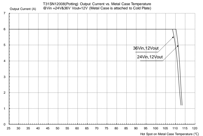
Figure 41: Output Current vs. Hot Spot on Metal Case Temperature @ V_{in}=24V\&36V , V_{out}=12V (Potting, Attach to Cold Plate)
