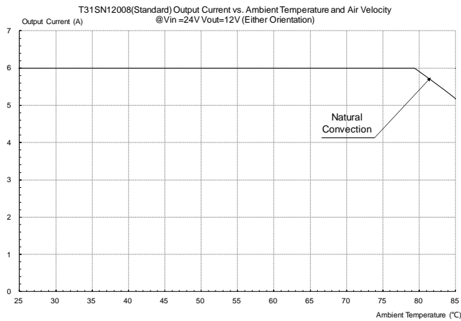
Figure 31: Output current vs. ambient temperature and air velocity @V in =24V, V out =12V (Either Orientation, Open Frame)
