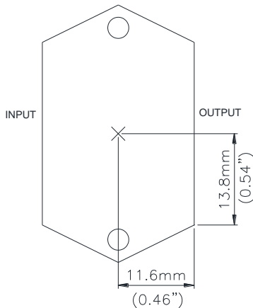
Figure 39: * Hot spot on metal case temperature measured point. The allowed maximum hot spot temperature is defined at 110°C.
