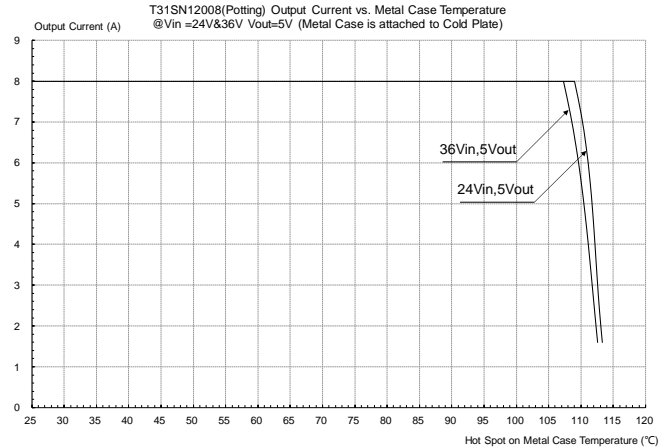
Figure 40: Output Current vs. Hot Spot on Metal Case Temperature @ V_{in}=24V\&36V , V_{out}=5V (Potting, Attach to Cold Plate)
