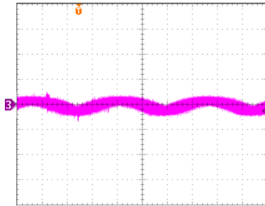
Figure 22: Input Reflected Ripple Current, i_s , through a 12\mu H source inductor at 48Vdc input voltage, 5Vdc output voltage and max load current (100mA/div, 1us/div).
