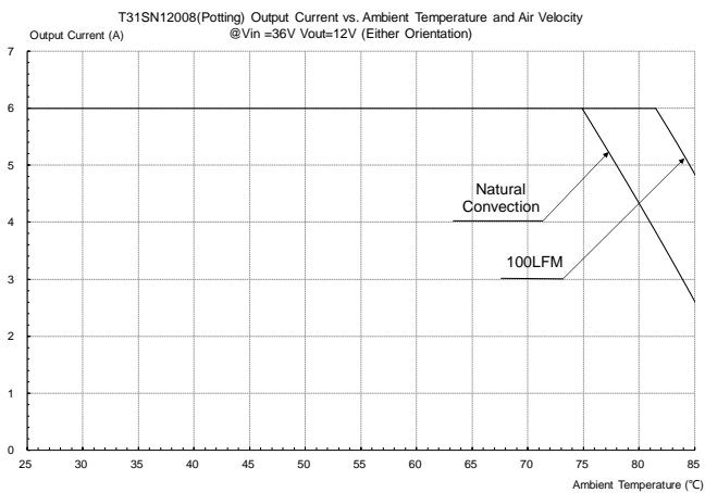
Figure 37: Output current vs. ambient temperature and air velocity @ V_{in}=36V , V_{out}=12V (Either Orientation, Potting)
