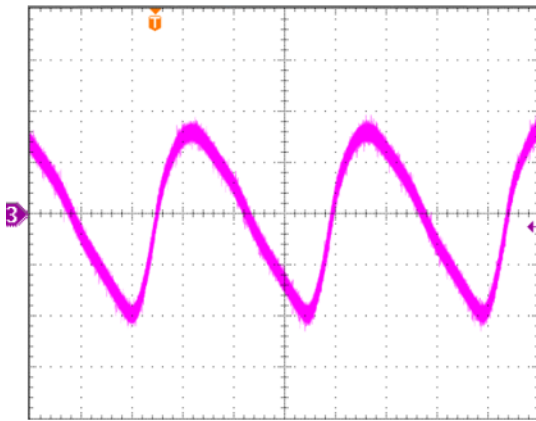
Figure 21: Input Terminal Ripple Current, i_c , at max output current, 5Vdc output voltage and 48Vdc input voltage with 12\mu H source impedance and 33\mu F electrolytic capacitor (100 mA/div, 1us/div).
