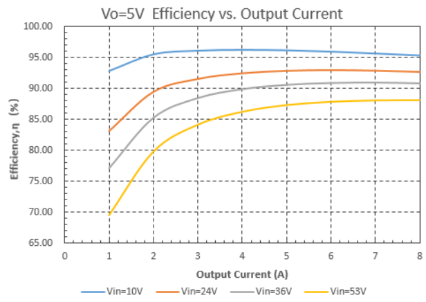
Figure 2: Efficiency vs. Output Current ( V_o=5\text{V} )
