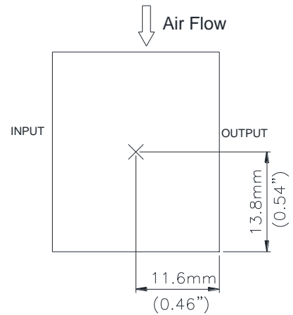
Figure 33: * Hot spot temperature measured point. The allowed maximum hot spot temperature is defined at 115°C.
