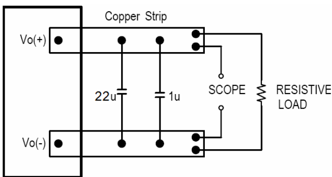
Figure 23: Test Setup for Output Voltage Noise and Ripple
