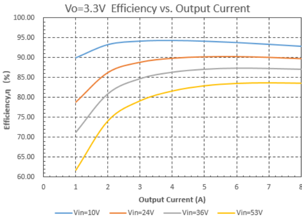
Figure 1: Efficiency vs. Output Current ( V_o=3.3\text{V} )
