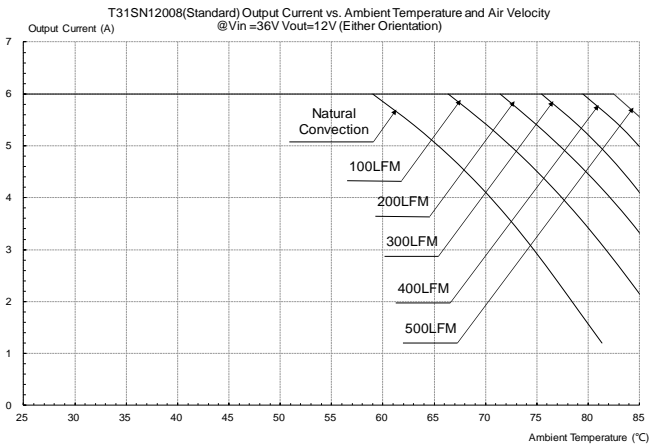
Figure 32: Output current vs. ambient temperature and air velocity @V in =36V, V out =12V (Either Orientation, Open Frame)
