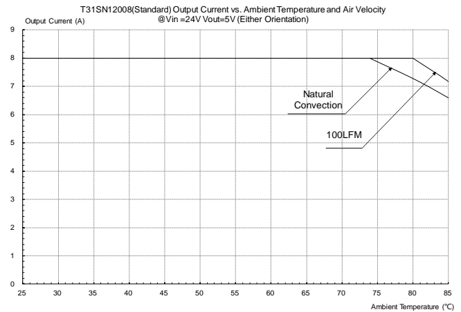
Figure 29: Output current vs. ambient temperature and air velocity @ V_{in}=24V , V_{out}=5V (Either Orientation, Open Frame)
