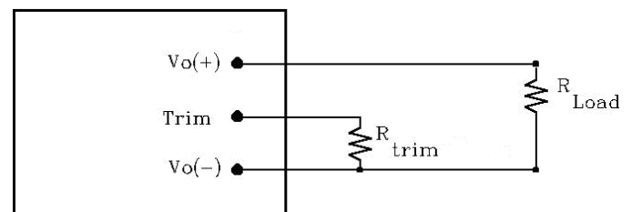
Figure 26: Circuit Configuration for Trim (decrease output voltage)
