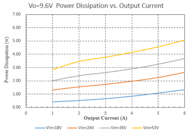
Figure 8: Power Dissipation vs. Output Current (Vo=9.6V)
