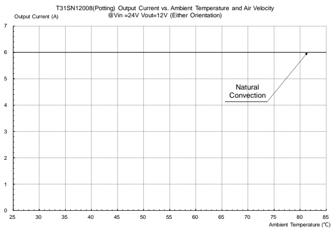
Figure 36: Output current vs. ambient temperature and air velocity @ V_{in}=24V , V_{out}=12V (Either Orientation, Potting)
