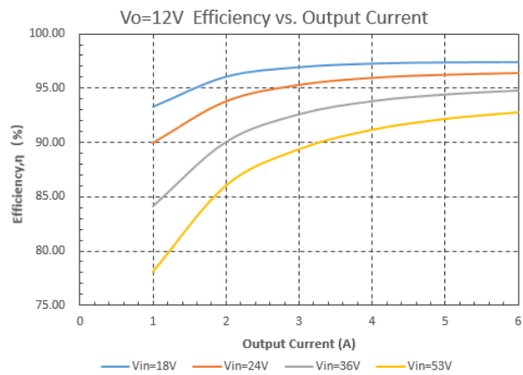
Figure 4: Efficiency vs. Output Current ( V_o=12\text{V} )
