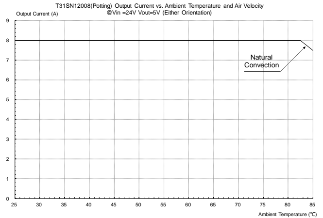
Figure 34: Output current vs. ambient temperature and air velocity @V in =24V, V out =5V (Either Orientation, Potting)
