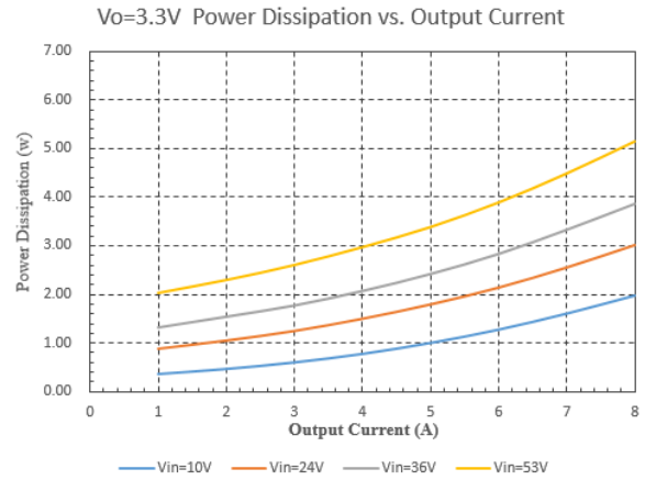
Figure 6: Power Dissipation vs. Output Current (Vo=3.3V)
