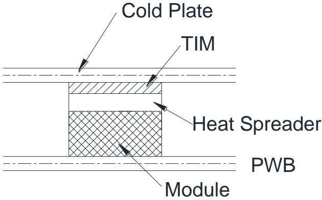
Figure 38: Cold Plate Cooling Test Setup
