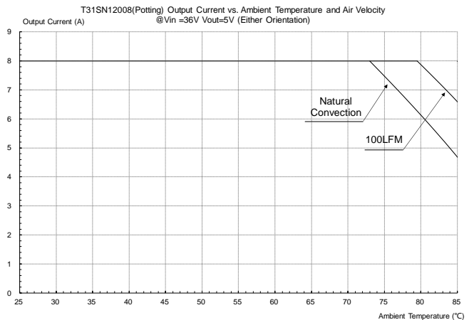
Figure 35: Output current vs. ambient temperature and air velocity @V in =36V, V out =5V (Either Orientation, Potting)
