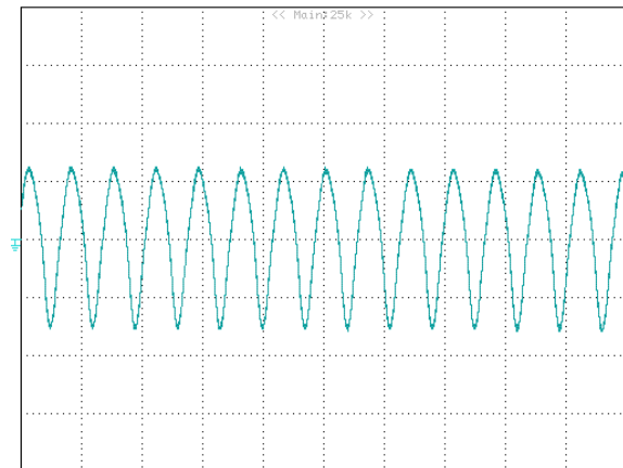
Figure 24: Output Voltage Ripple and Noise at 48Vdc input voltage, 12Vdc output voltage and max load current (20 mV/div, 5us/div) Load cap: 1\mu F ceramic capacitor and 22\mu F ceramic capacitor. Bandwidth: 20MHz
