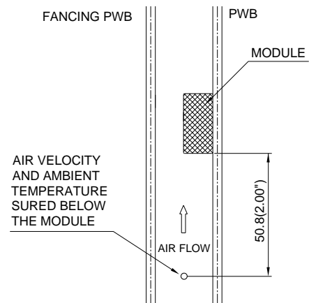
Figure 17: Wind tunnel test setup
