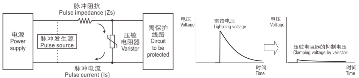
壓敏電阻器對脈衝的吸收 PULSE ABSORPTION BY VARISTOR
