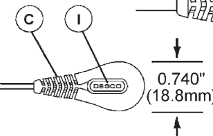
RESISTOR END
