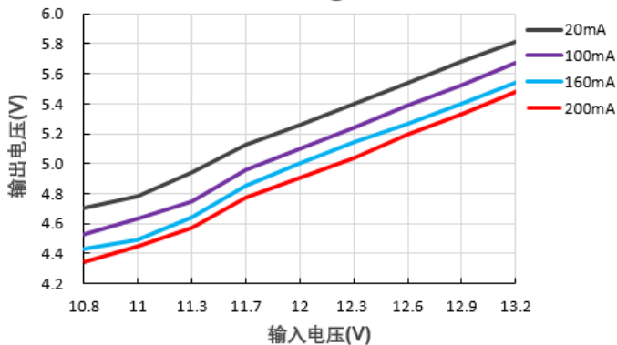
输出电压Vs输入电压@B1205S-1WR2
