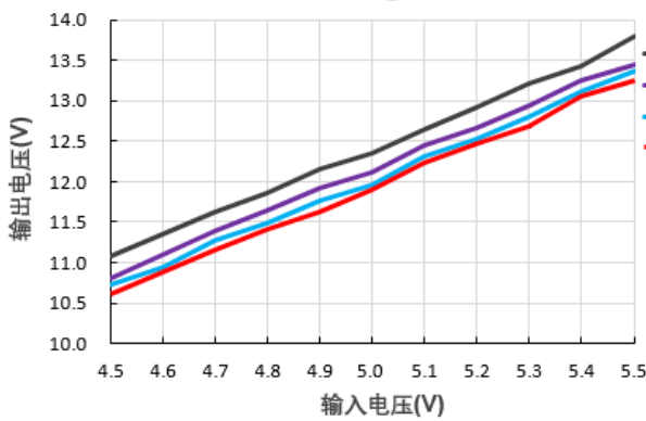
输出电压Vs输入电压@B0512LS-1WR3
