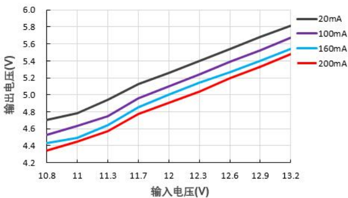
输出电压 VS 输入电压 (B1205S-1W)
