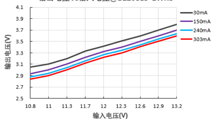
输出电压Vs输入电压@B1203LS-1WR3
