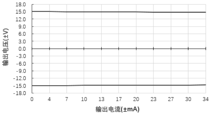
输出电压Vs输出电流(Vin=12V)@E2415S-1WR2
