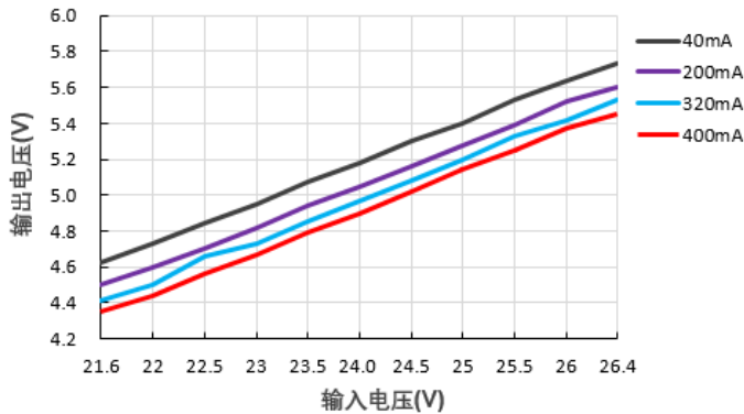
输出电压Vs输入电压@F2405S-2WR2
