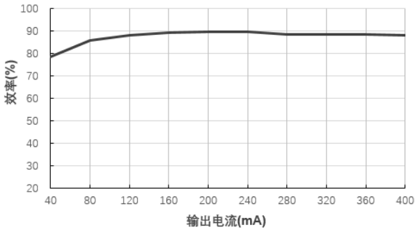
效率Vs输出电流(Vin=24V)@F2405S-2WR2
