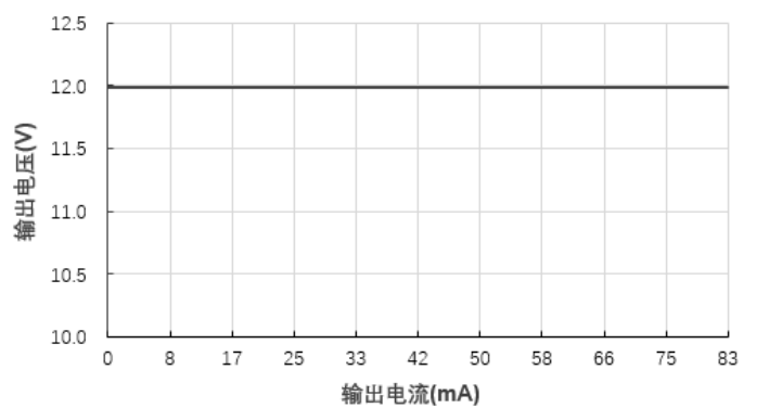
输出电压Vs输出电流(Vin=12V)@IB1212LS-1WR3
