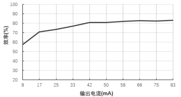
效率Vs输出电流(Vin=12V)@IB1212LS-1WR3
