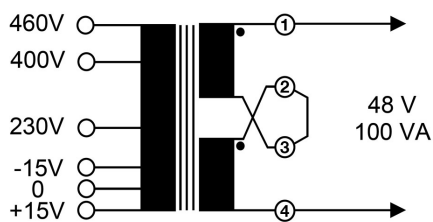
SERIAL CONNECTION
