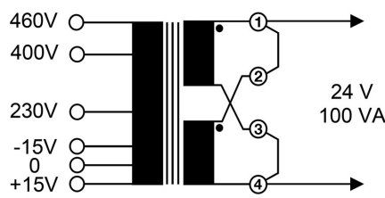
PARALLEL CONNECTION
