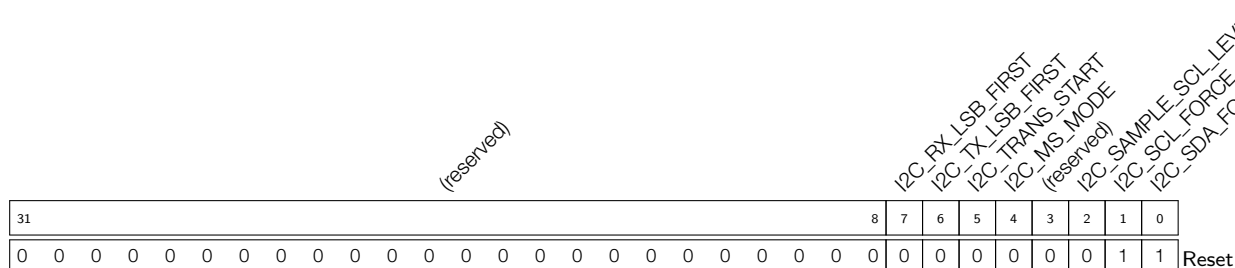
Register 11.2: I2C_CTR_REG (0x0004)
