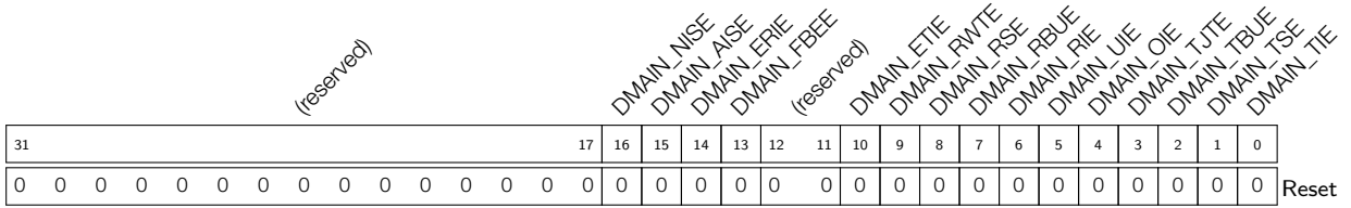
Register 10.8: DMAIN_EN_REG (0x001C)
