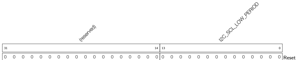
Register 11.1: I2C_SCL_LOW_PERIOD_REG (0x0000)
