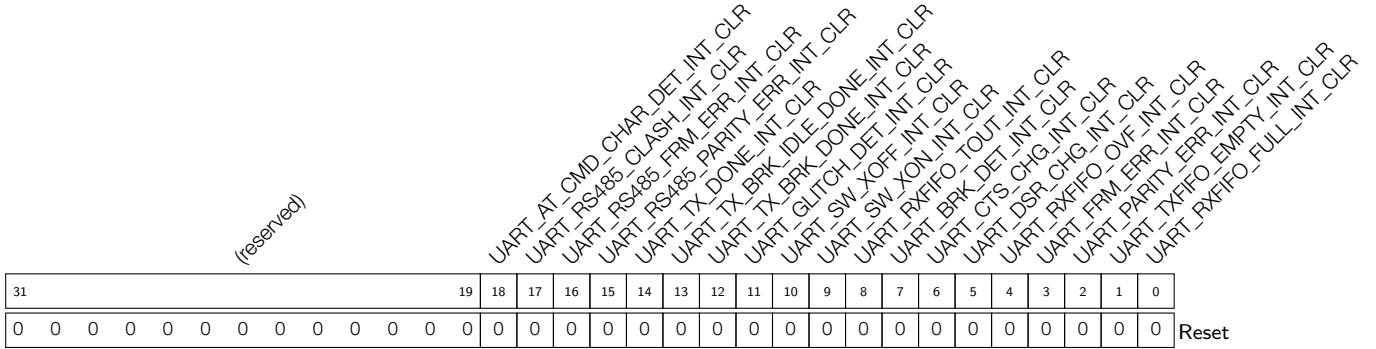
Register 13.5: UART_INT_CLR_REG (0x10)
