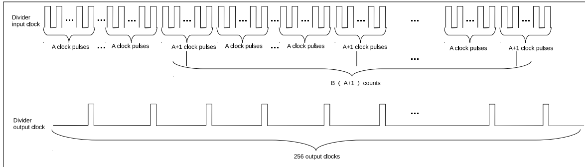
Figure 89: LED_PWM Divider
