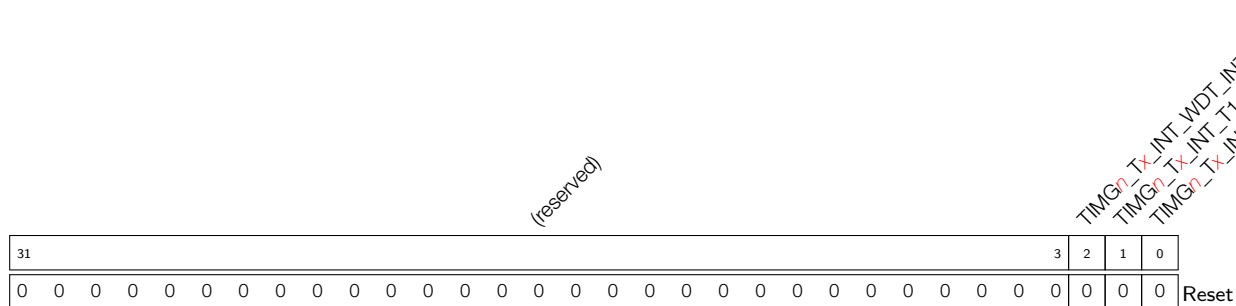
Register 18.21: TIMG n _Tx_INT_RAW_REG (0x009c)
