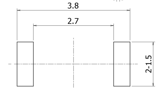
PCB SOLDER LAND DIMENSIONS
