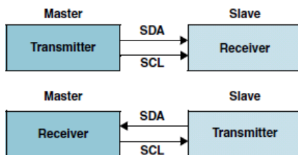
Figure 80: Master/Slave and Transmitter/Receiver Relationships
