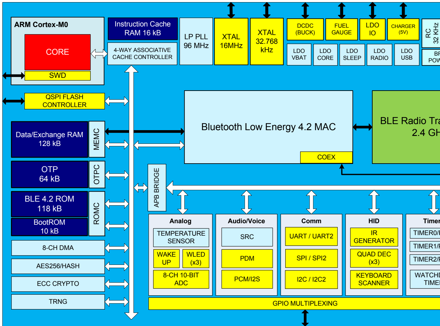
Figure 1: DA14681 block diagram
